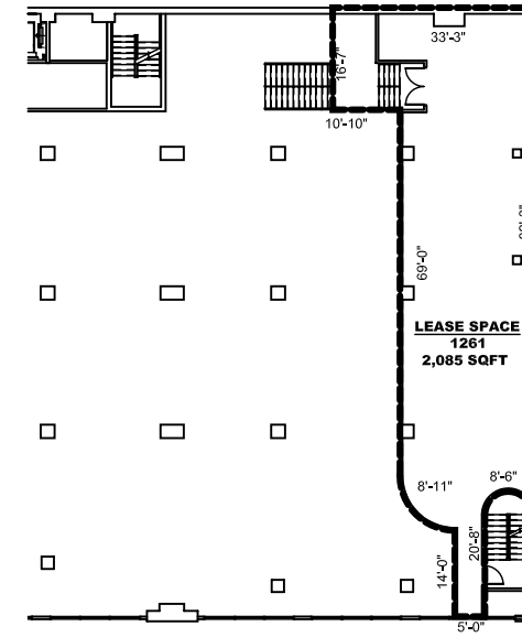
MEZZANINE LEASE PLAN SCALE - 1/16" = 1'-0"
